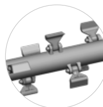
Standard rotor with SMW flails
