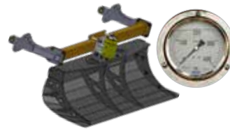
Grader blade (option), hydr. height and rotation adjustment, with hydraulic pneumatic damping incl. lateral extensions · pressure gauge to control work of the grader blade
